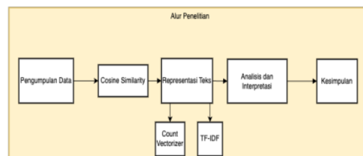
Gambar 1. Alur Penelitian
